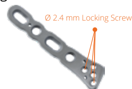
Locking Distal Ulna Plate
